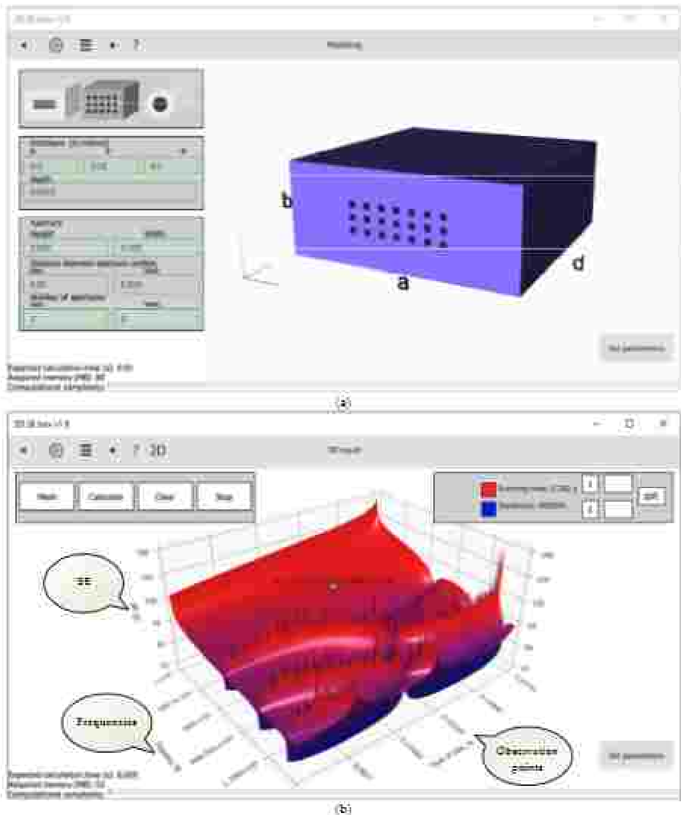
Figure 26. GUI of the software prototype: setting the microwaves geometry (a), displaying the three-dimensional pattern of the SE (b).
