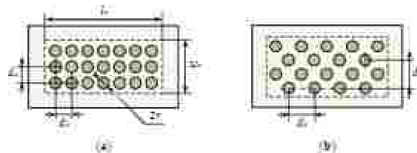
Figure 4. Enclosure front wall perforated with circular apertures: (a) array of regular apertures; (b) array of staggered apertures.
