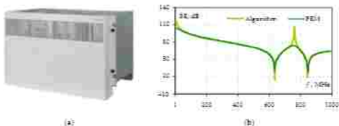
Figure 23. Enclosure of the ABB PDX 515 multiplexer (a) and frequency dependencies of its SE (b).
