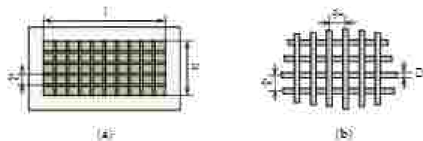
Figure 3. The aperture populated with wire grid (a) and geometry of this wire grid (b).
