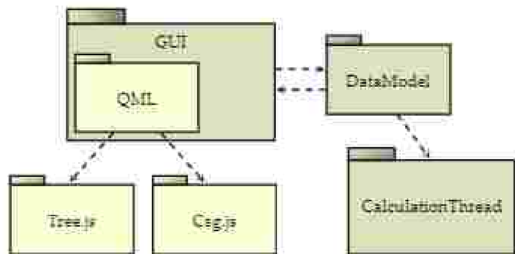
Figure 28. Software architecture as a UML package diagram.
