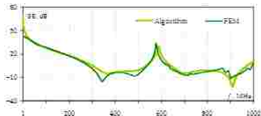
Figure 24. Frequency dependence of the SE for the cylindrical enclosure filled with dielectrics.
