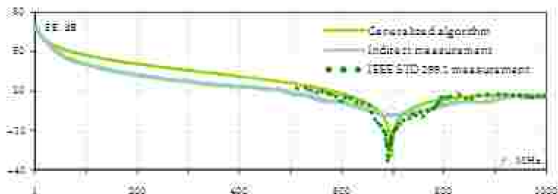
Figure 20. Frequency dependence of the SE for the empty enclosure with a square aperture.
