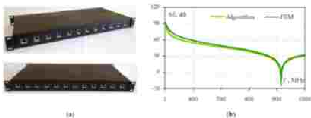
Figure 22. Shielding enclosure of the Ethernet filter (a) and frequency dependencies of its SE (b).
