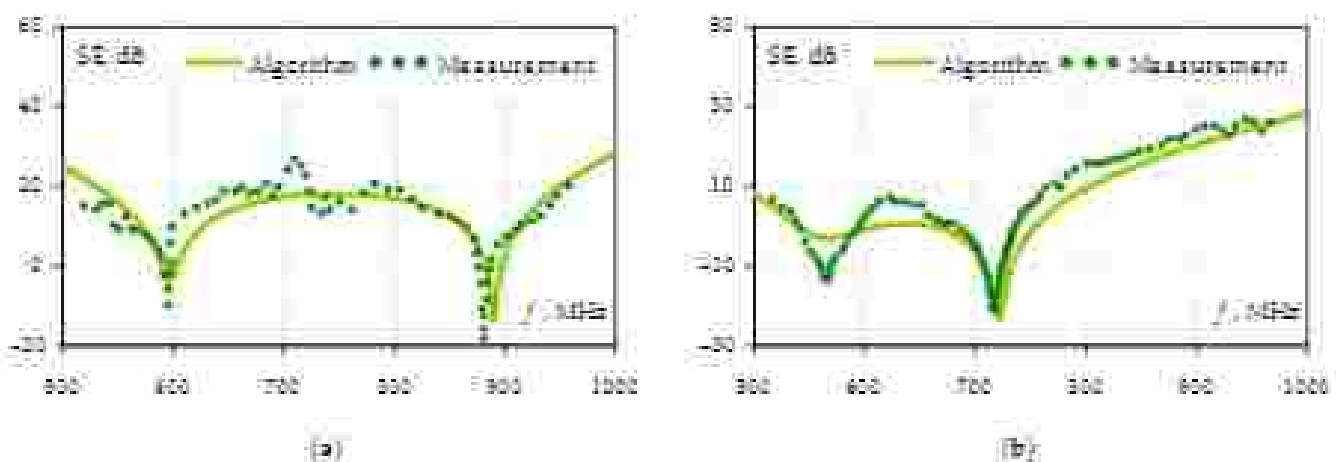
Figure 21. Frequency dependence of the SE for enclosures from cases 2 (a) and 5 (b).
