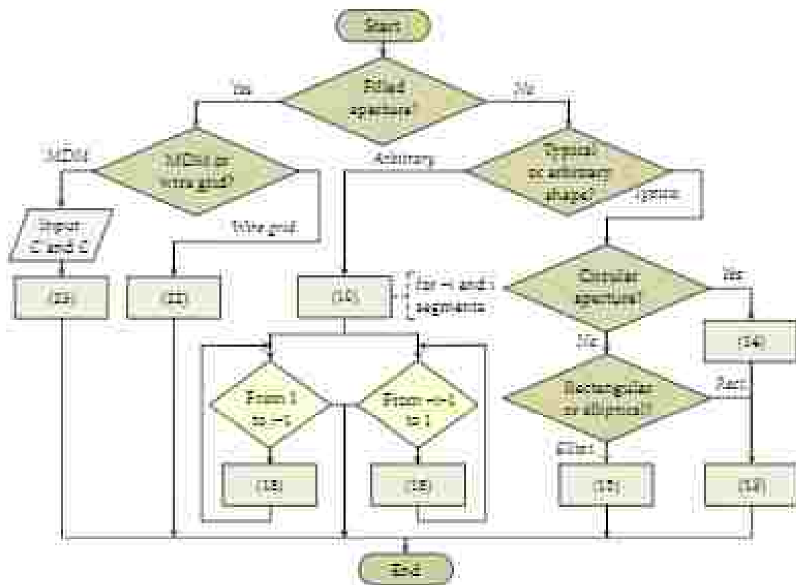
Figure 11. Algorithm of Z_{sp} calculation for a single aperture (Flowchart 2).
