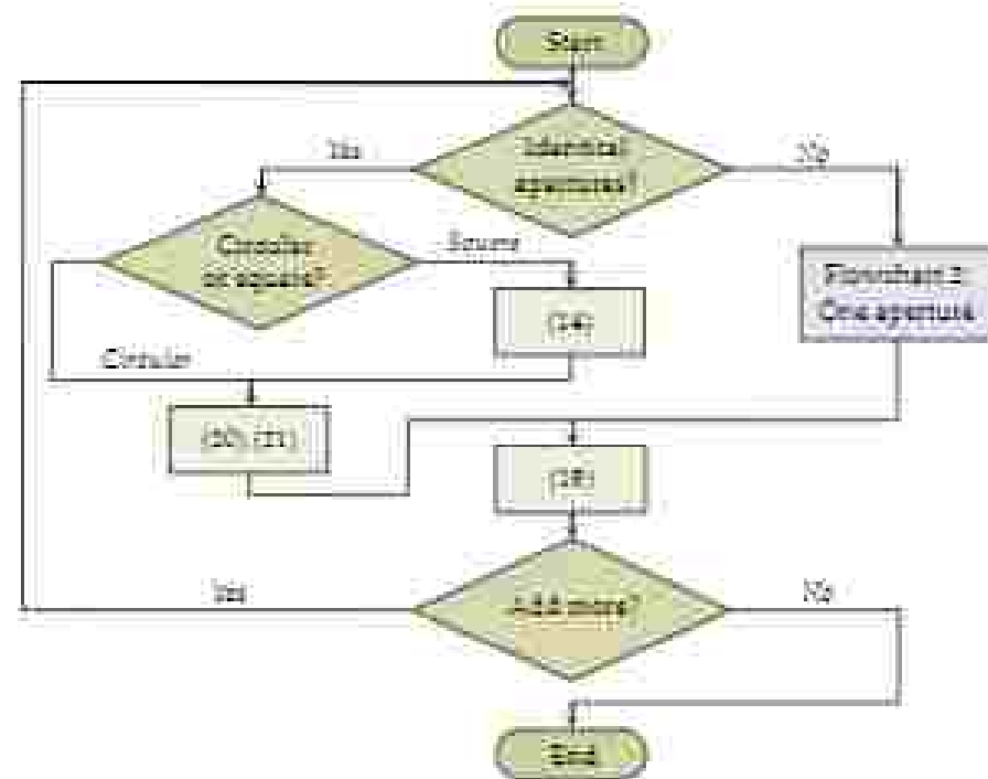
Figure 13. Algorithm of Z_{eq} calculation for a group of apertures (Flowchart 4).
