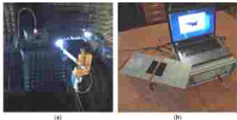
Figure 19. Test setups for measuring SE according to IEEE STD 299.1 (a) and using the indirect method (b).
